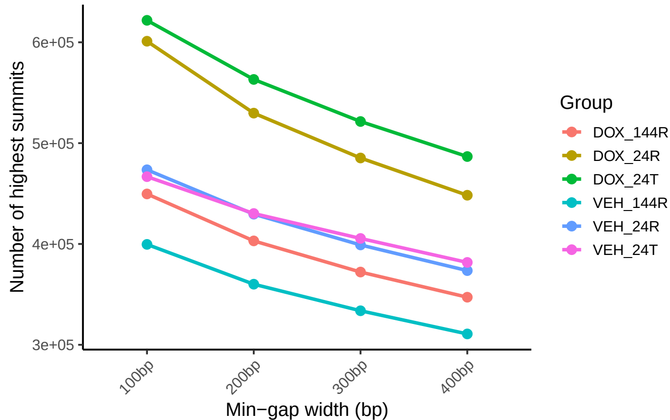
Effect of min-gap width on number of highest summits per group; H3K36me3
